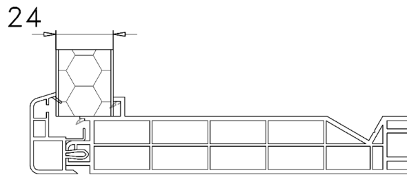
Misure pannello
